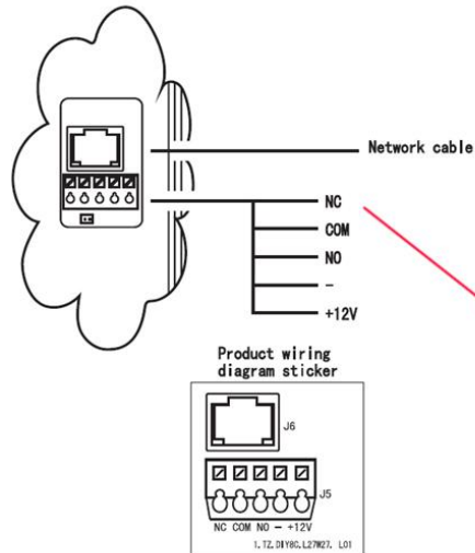
Wiring diagram
